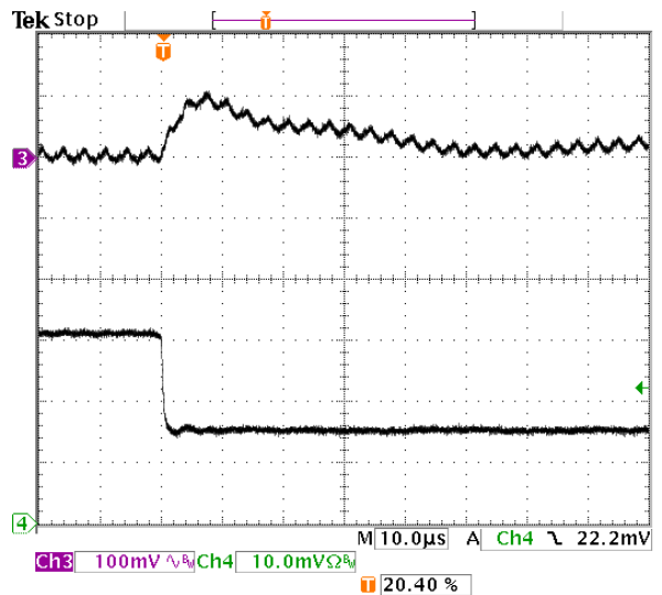
Fig-3.3V-7: Output voltage response for V_{out}=3.3V to negative load current step-change from 6A to 3A with slew rate of -5A/\mu s at V_{in}=5.0V . C_o=47\mu F \times 2 ceramic. Top trace: output voltage (100mV/div.) Bottom trace: load current (2A/div.) Time scale: 10µs/div.
