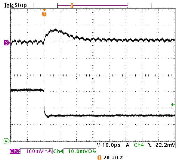
Fig-1.0V-7: Output voltage response for V_{out}=1.0V to positive load current step-change from 6A to 3A with slew rate of -5A/\mu s at V_{in}=5.0V . C_o=47\mu F \times 2 ceramic. Top trace: output voltage (100mV/div.) Bottom trace: load current (2A/div.) Time scale: 10μs/div.
