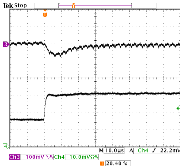
Fig-1.0V-6: Output voltage response for V_{out}=1.0V to positive load current step-change from 3A to 6A with slew rate of 5A/\mu s at V_{in}=5.0V . C_o=47\mu F \times 2 ceramic. Top trace: output voltage (100mV/div.) Bottom trace: load current (2A/div.) Time scale: 10μs/div.
