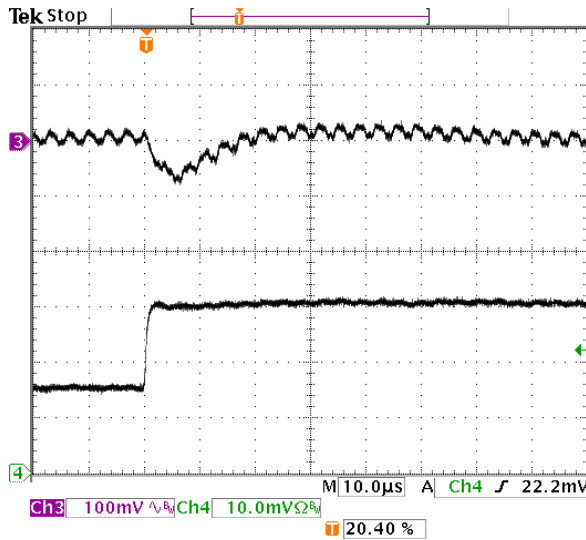
Fig-1.8V-6: Output voltage response for V_{out}=1.8V to positive load current step-change from 3A to 6A with slew rate of 5A/\mu s at V_{in}=5.0V . C_o=47\mu F \times 2 ceramic. Top trace: output voltage (100mV/div.) Bottom trace: load current (2A/div.) Time scale: 10μs/div.
