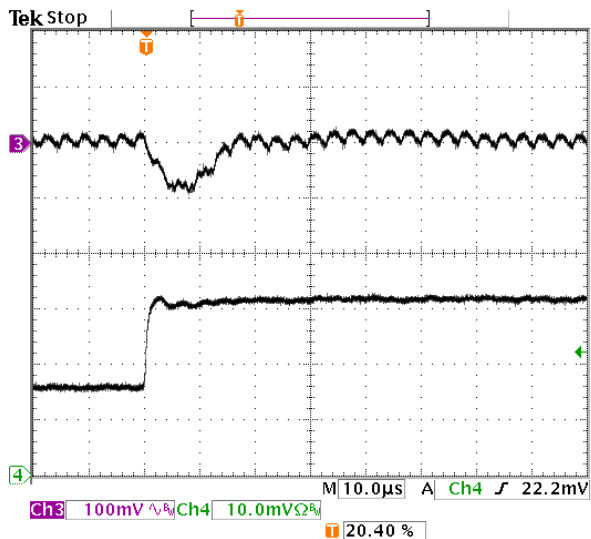
Fig-1.5V-6: Output voltage response for V_{out}=1.5V to positive load current step-change from 3A to 6A with slew rate of 5A/\mu s at V_{in}=5.0V . C_o=47\mu F \times 2 ceramic. Top trace: output voltage (100mV/div.) Bottom trace: load current (2A/div.) Time scale: 10μs/div.
