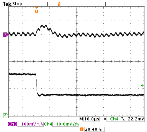
Fig-1.8V-7: Output voltage response for V_{out}=1.8V to positive load current step-change from 6A to 3A with slew rate of -5A/\mu s at V_{in}=5.0V . C_o=47\mu F \times 2 ceramic. Top trace: output voltage (100mV/div.) Bottom trace: load current (2A/div.) Time scale: 10μs/div.
