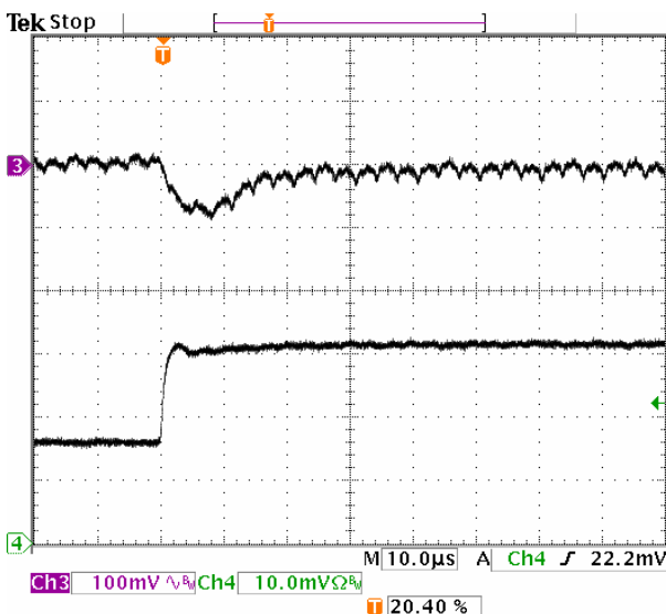
Fig-0.7525V-6: Output voltage response for V_{out}=0.7525V to positive load current step-change from 3A to 6A with slew rate of 5A/\mu s at V_{in}=5.0V . C_o=47\mu F \times 2 ceramic. Top trace: output voltage (100mV/div.) Bottom trace: load current (2A/div.) Time scale: 10μs/div.
