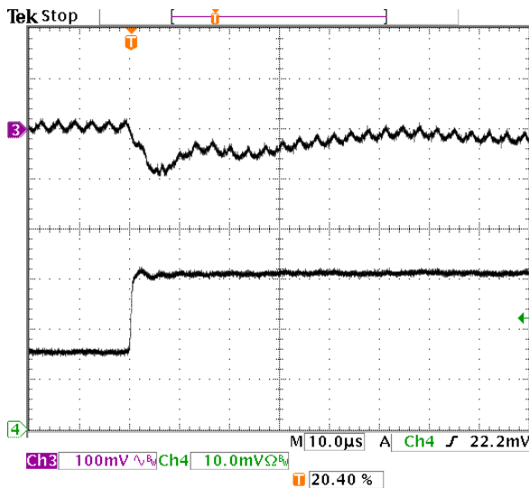
Fig-3.3V-6: Output voltage response for V_{out}=3.3V to positive load current step-change from 3A to 6A with slew rate of 5A/\mu s at V_{in}=5.0V . C_o=47\mu F \times 2 ceramic. Top trace: output voltage (100mV/div.) Bottom trace: load current (2A/div.) Time scale: 10µs/div.
