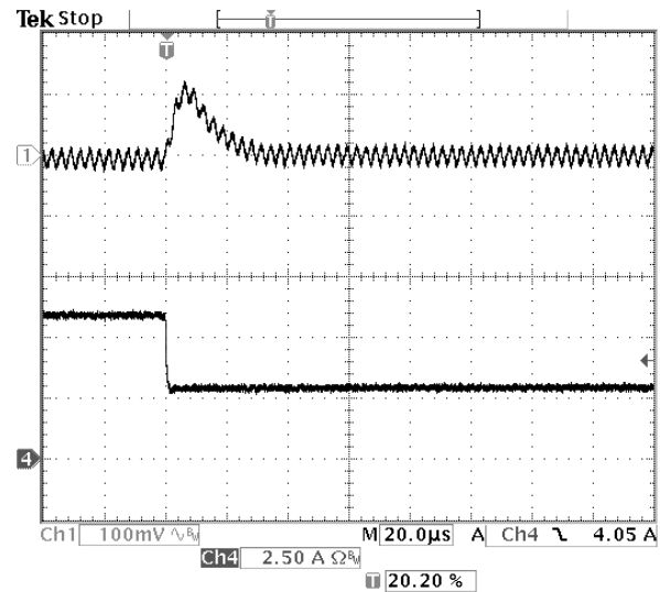
Fig-5.0V-7: Output voltage response for V_{out}=5.0V to negative load current step-change from 6A to 3A with slew rate of -5A/\mu s at V_{in}=12.0V . C_o=47\mu F \times 2 ceramic.
