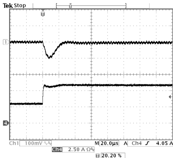
Fig-1.0V-6: Output voltage response for V_{out}=1.0V to positive load current step-change from 3A to 6A with slew rate of 5A/\mu s at V_{in}=12.0V . C_o=47\mu F \times 2 ceramic.
