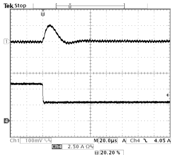
Fig-1.0V-7: Output voltage response for V_{out}=1.0V to negative load current step-change from 6A to 3A with slew rate of -5A/\mu s at V_{in}=12.0V . C_o=47\mu F \times 2 ceramic.
