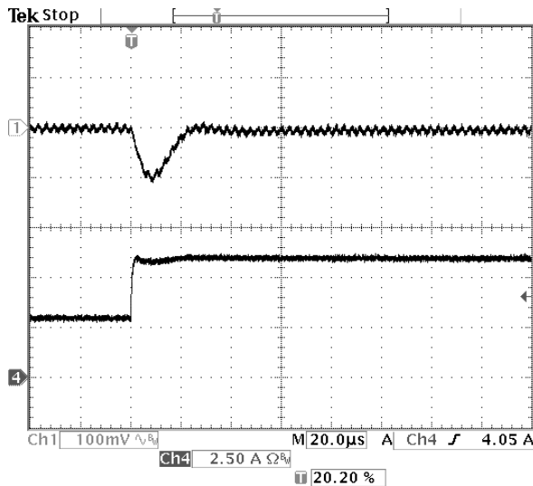
Fig-1.5V-6: Output voltage response for V_{out}=1.5V to positive load current step-change from 3A to 6A with slew rate of 5A/\mu s at V_{in}=12.0V . C_o=47\mu F \times 2 ceramic.
