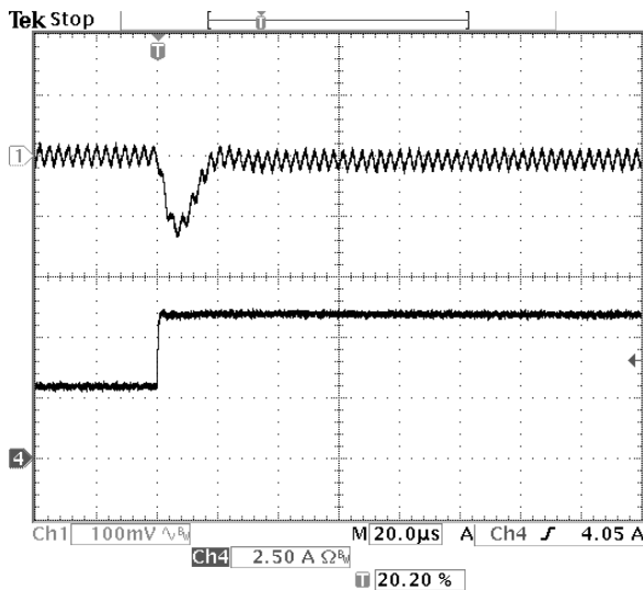
Fig-5.0V-6: Output voltage response for V_{out}=5.0V to positive load current step-change from 3A to 6A with slew rate of 5A/\mu s at V_{in}=12.0V . C_o=47\mu F \times 2 ceramic.
