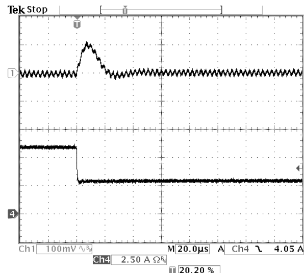
Fig-2.5V-7: Output voltage response for V_{out}=2.5V to negative load current step-change from 6A to 3A with slew rate of -5A/\mu s at V_{in}=12.0V . C_o=47\mu F \times 2 ceramic.
