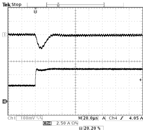
Fig-1.2V-6: Output voltage response for V_{out}=1.2V to positive load current step-change from 3A to 6A with slew rate of 5A/\mu s at V_{in}=12.0V . C_o=47\mu F \times 2 ceramic.
