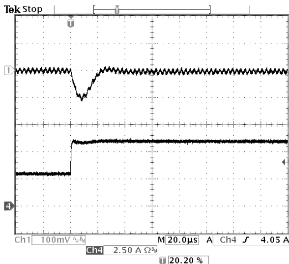
Fig-2.0V-6: Output voltage response for V_{out}=2.0V to positive load current step-change from 3A to 6A with slew rate of 5A/\mu s at V_{in}=12.0V . C_o=47\mu F \times 2 ceramic.
