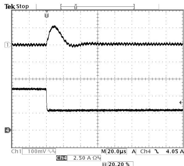
Fig-1.2V-7: Output voltage response for V_{out}=1.2V to negative load current step-change from 6A to 3A with slew rate of -5A/\mu s at V_{in}=12.0V . C_o=47\mu F \times 2 ceramic.
