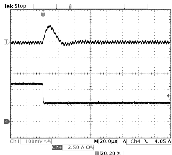
Fig-2.0V-7: Output voltage response for V_{out}=2.0V to negative load current step-change from 6A to 3A with slew rate of -5A/\mu s at V_{in}=12.0V . C_o=47\mu F \times 2 ceramic.
