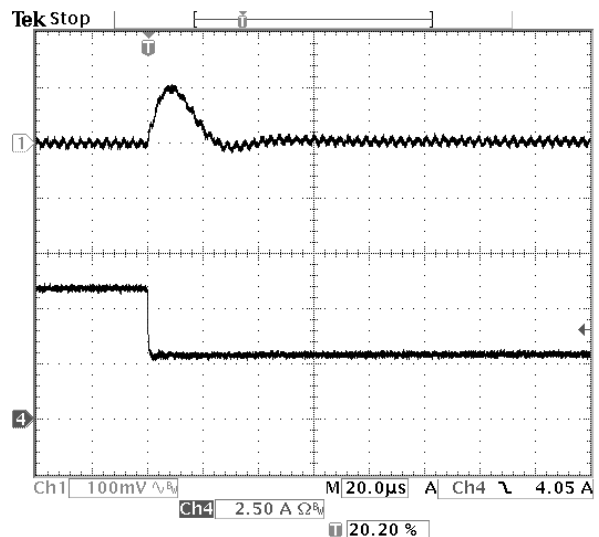
Fig-1.5V-7: Output voltage response for V_{out}=1.5V to negative load current step-change from 6A to 3A with slew rate of -5A/\mu s at V_{in}=12.0V . C_o=47\mu F \times 2 ceramic.
