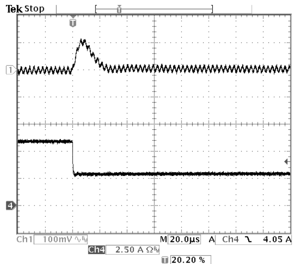
Fig-3.3V-7: Output voltage response for V_{out}=3.3V to negative load current step-change from 6A to 3A with slew rate of -5A/\mu s at V_{in}=12.0V . C_o=47\mu F \times 2 ceramic.
