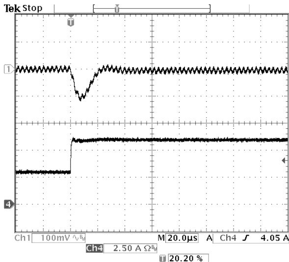
Fig-2.5V-6: Output voltage response for V_{out}=2.5V to positive load current step-change from 3A to 6A with slew rate of 5A/\mu s at V_{in}=12.0V . C_o=47\mu F \times 2 ceramic.
