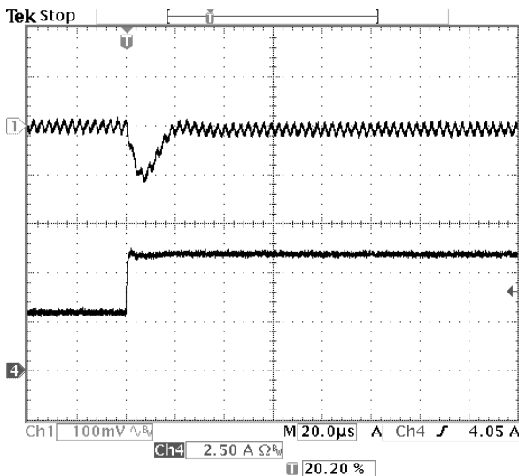
Fig-3.3V-6: Output voltage response for V_{out}=3.3V to positive load current step-change from 3A to 6A with slew rate of 5A/\mu s at V_{in}=12.0V . C_o=47\mu F \times 2 ceramic.
