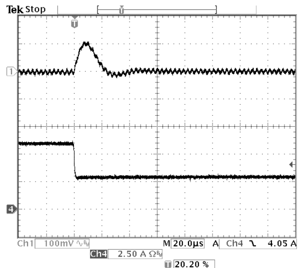
Fig-1.8V-7: Output voltage response for V_{out}=1.8V to negative load current step-change from 6A to 3A with slew rate of -5A/\mu s at V_{in}=12.0V . C_o=47\mu F \times 2 ceramic.
