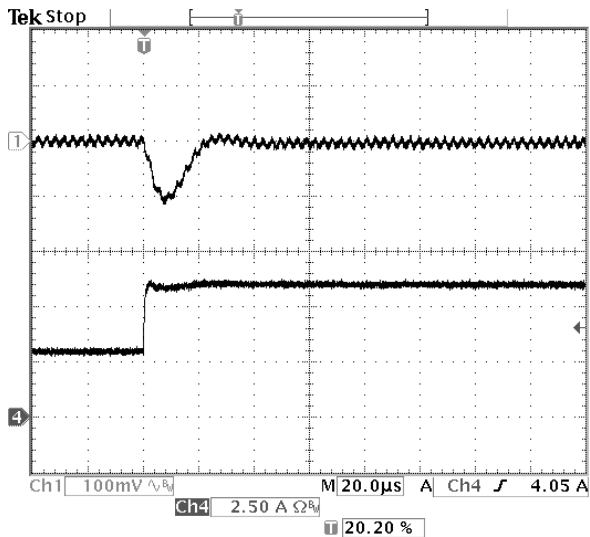
Fig-1.8V-6: Output voltage response for V_{out}=1.8V to positive load current step-change from 3A to 6A with slew rate of 5A/\mu s at V_{in}=12.0V . C_o=47\mu F \times 2 ceramic.
