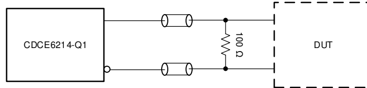
Figure 8-12. LVDS Output - DC-Coupled. Place 100 \Omega close to the DUT
