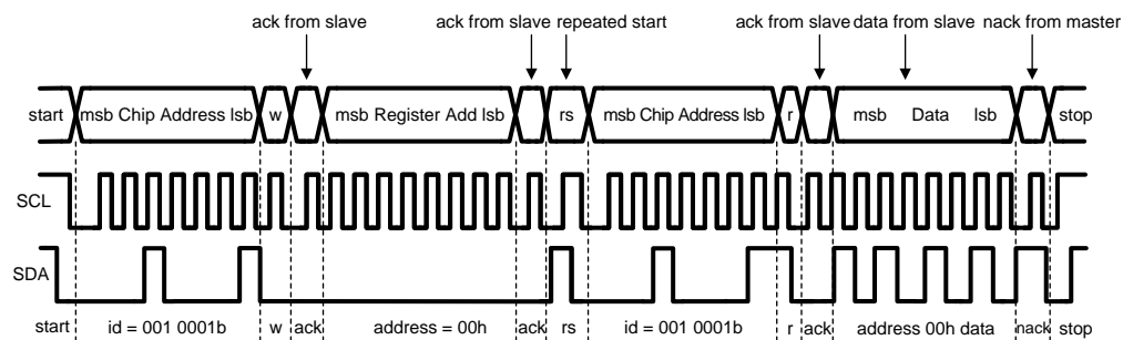
Figure 47. Register Read Format
