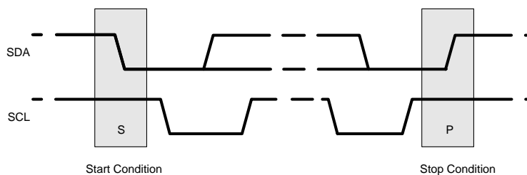
Figure 33. Start and Stop Conditions
