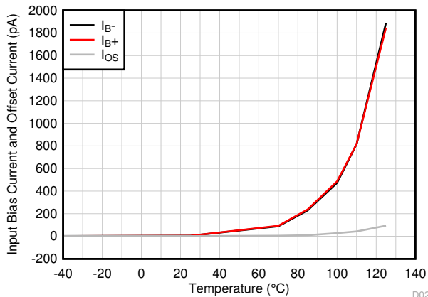
Figure 6-14. Input Bias Current and Offset Current vs Temperature
