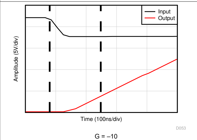
Figure 6-36. Negative Overload Recovery
