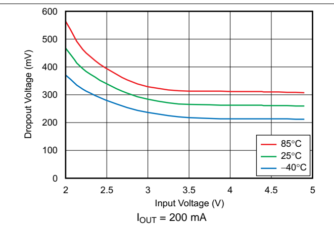
Figure 14. Dropout Voltage vs Input Voltage
