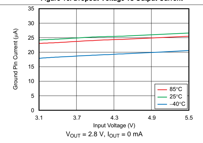
Figure 18. Ground Pin Current vs Input Voltage
