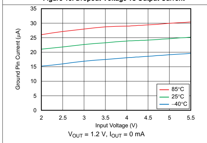
Figure 17. Ground Pin Current vs Input Voltage
