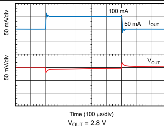
Figure 42. Load Transient Response
