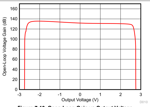
Figure 7-10. Open-Loop Gain vs Output Voltage
