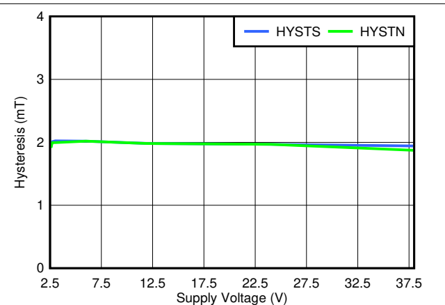
Figure 7-6. TMAG5123B Hysteresis vs Supply Voltage
