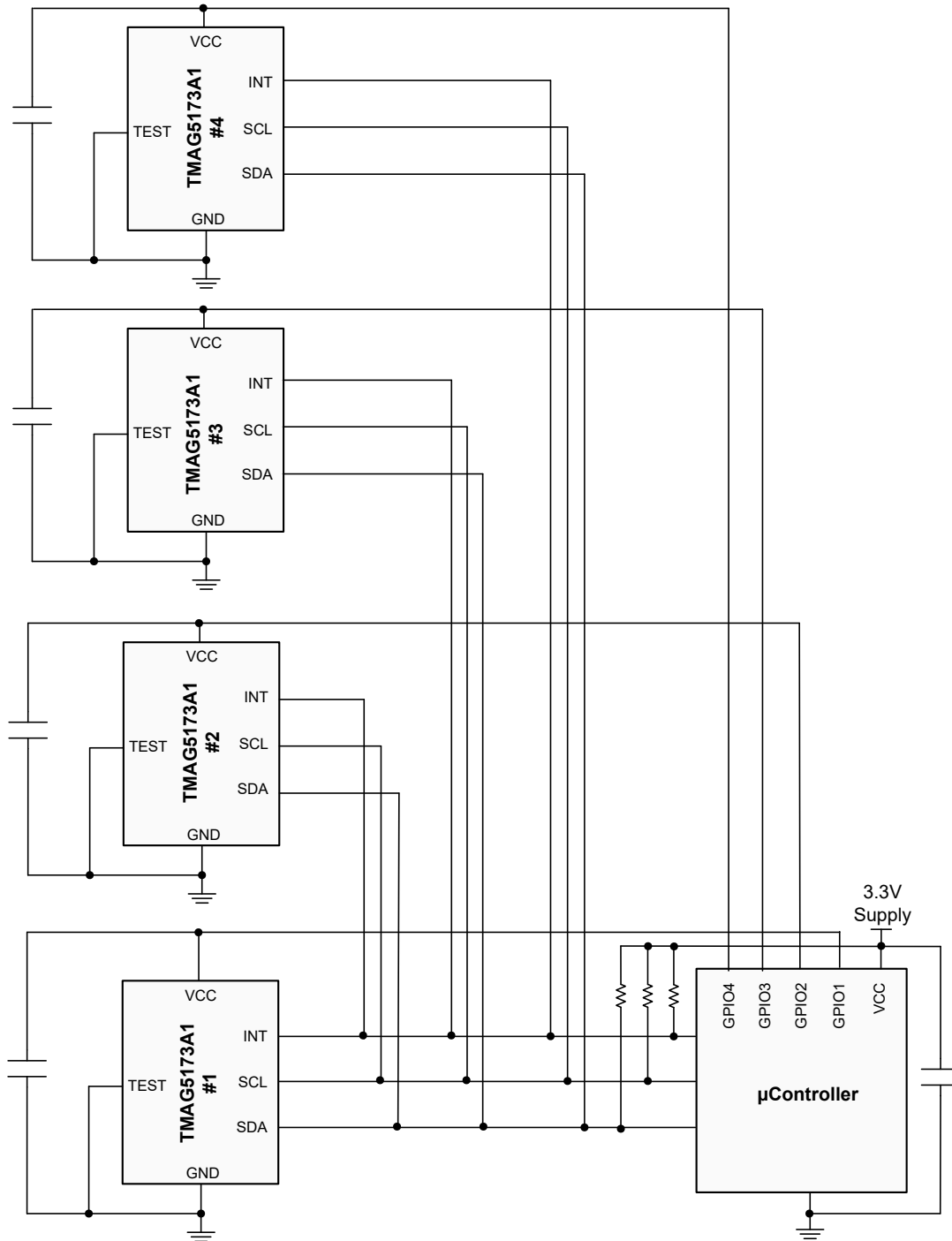
Figure 8-8. TMAG5173-Q1 Application Diagram for I 2 C Address Expansion
