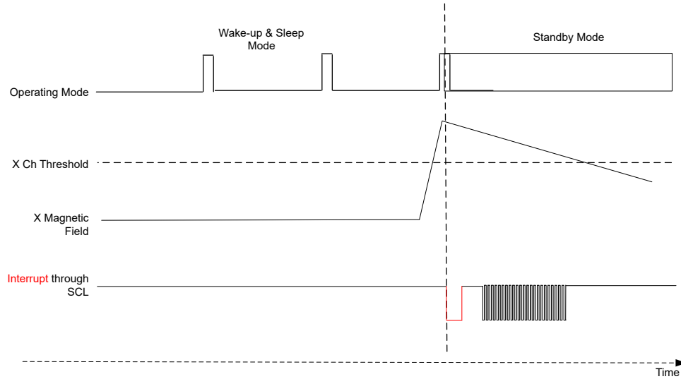
Figure 7-3. Interrupt Through SCL
