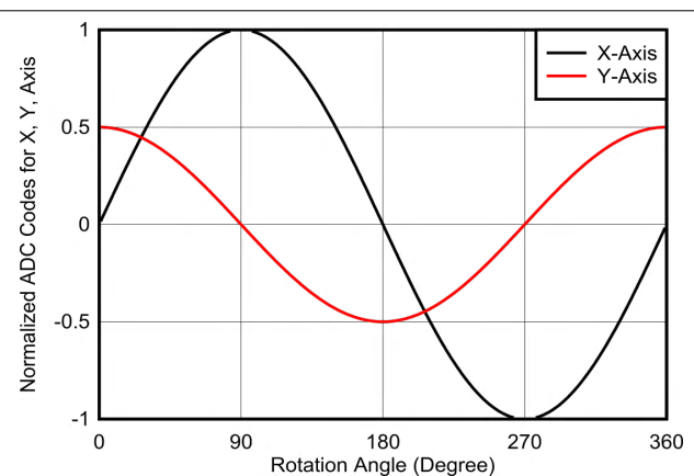
Figure 8-13. X and Y Sensor Data for Full 360 Degree Rotation for Off-Axis Measurement
