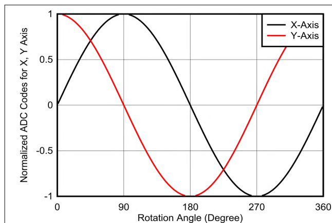
Figure 8-12. X and Y Sensor Data for Full 360 Degree Rotation for On-Axis Measurement
