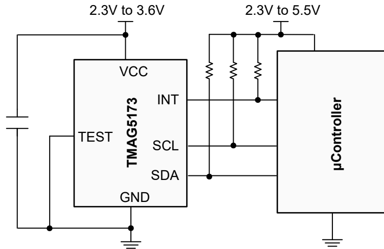
Figure 8-10. TMAG5173-Q1 Application Diagram for Angle Measurement
