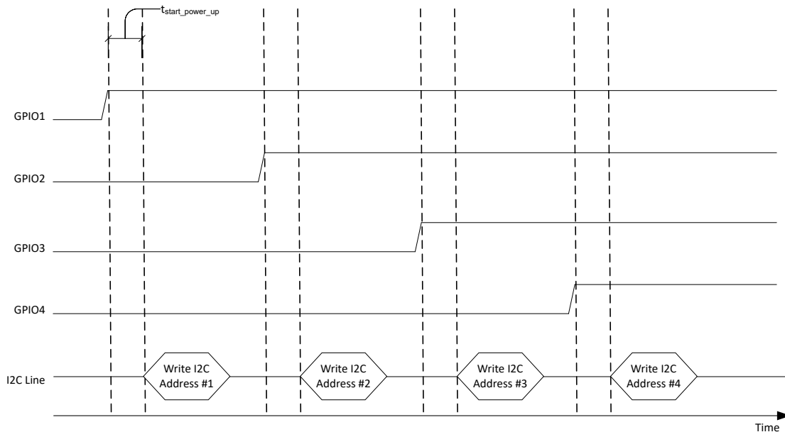
Figure 8-9. Power-Up Timing and I 2 C Address Allocation for the Four Sensors
