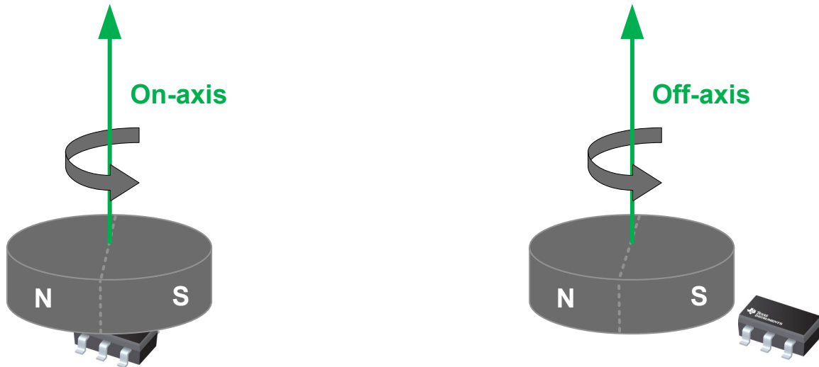
Figure 8-11. On-Axis vs Off-Axis Angle Measurements
