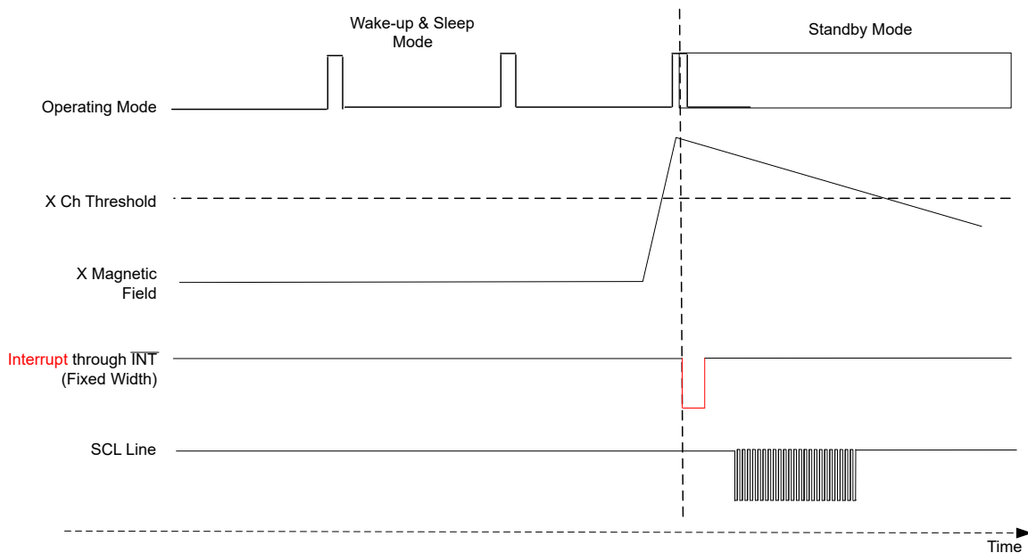
Figure 7-4. Fixed Width Interrupt Through \overline{\text{INT}}
