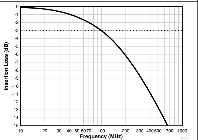
Figure 7-16. CC Bandwidth
