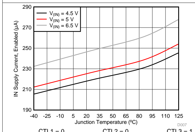
Figure 7. Enabled IN Supply Current – DCP_Auto (001) vs Temperature
