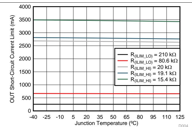
Figure 4. OUT Short-Circuit Current Limit vs Temperature
