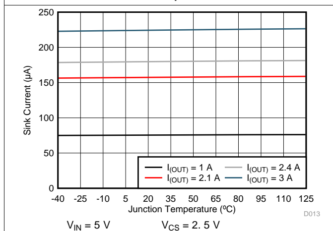
Figure 13. I_{CS} vs Temperature
