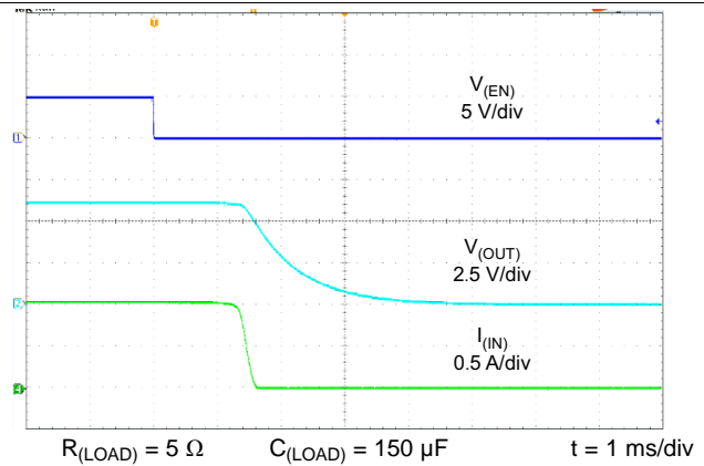
Figure 21. Turnoff Response
