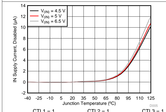
Figure 5. Disabled IN Supply Current vs Temperature
