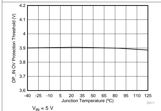
Figure 11. DP_IN Overvoltage Protection Threshold vs Temperature
