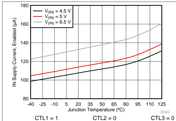
Figure 9. Enabled IN Supply Current – Client Mode (100) vs Temperature
