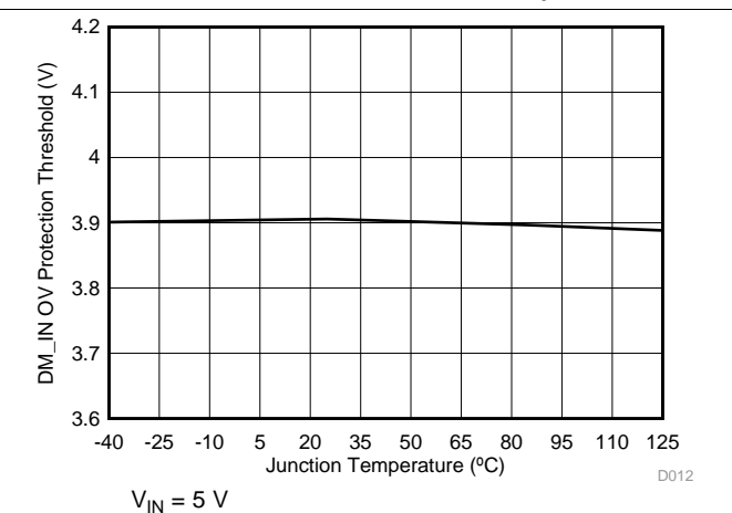
Figure 12. DM_IN Overvoltage Protection Threshold vs Temperature
