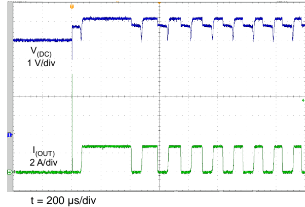
Figure 57. V_{BUS} Shorted to GND, V_{(DC)}
