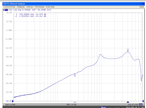
Figure 33. Data Transmission Characteristics vs Frequency
