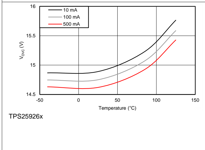
Figure 5. V_OVC vs Temperature Across I_OUT
