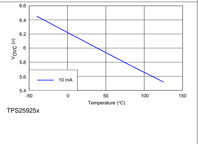
Figure 6. V_OVC vs Temperature
