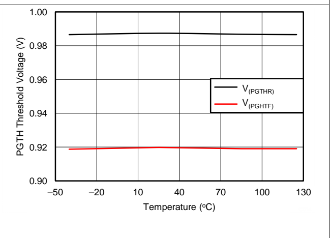
Figure 6. PGTH Threshold Voltage vs Temperature
