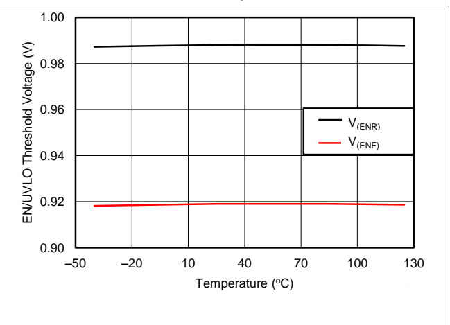
Figure 4. EN Threshold Voltage vs Temperature
