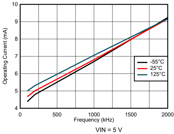
Figure 7-1. Operating Current Variation
