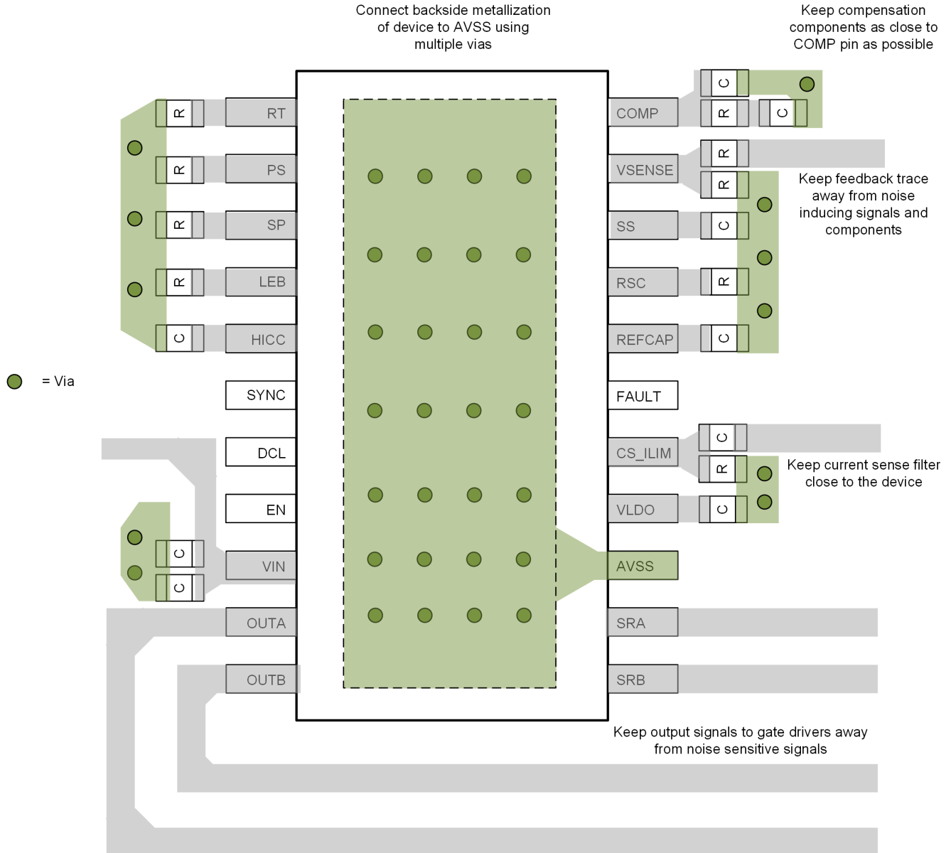
Figure 9-4. PCB Layout Example
