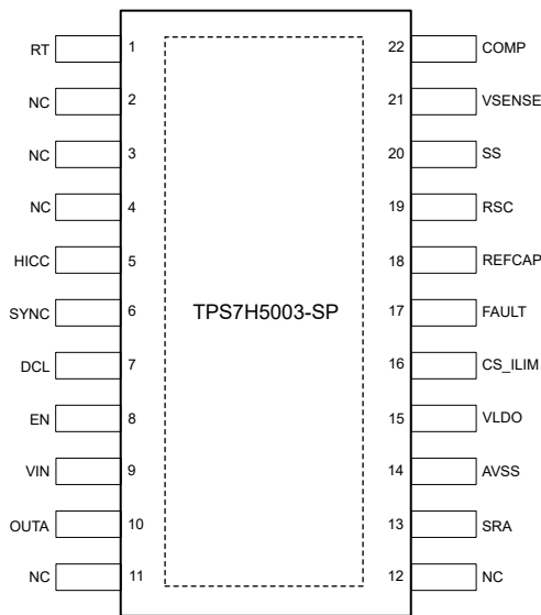
Figure 6-3. TPS7H5003-SP HFT Package 22-Pin CFP With Thermal Pad (Top View)
