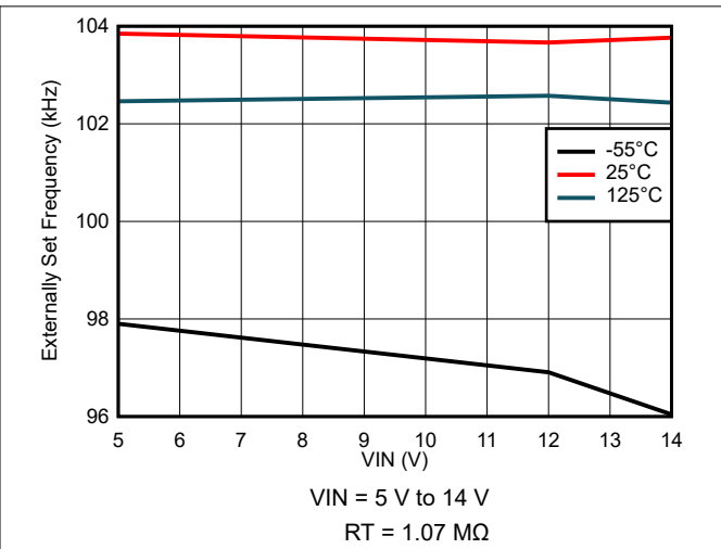
Figure 7-20. Externally Set Frequency Variation
