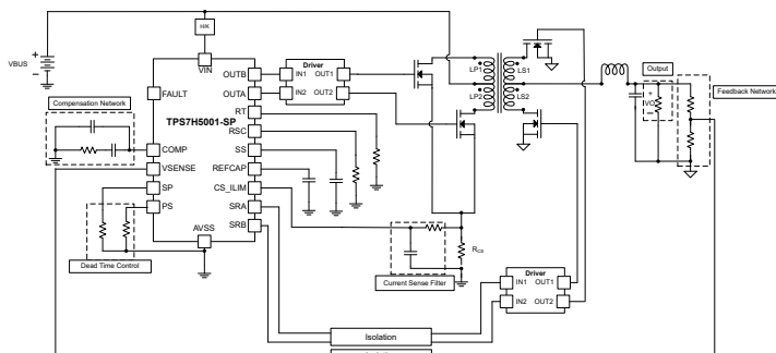
Typical Application for TPS7H5001-SP
