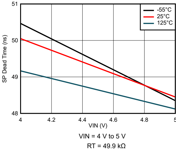
Figure 7-51. SP Dead Time Variation
