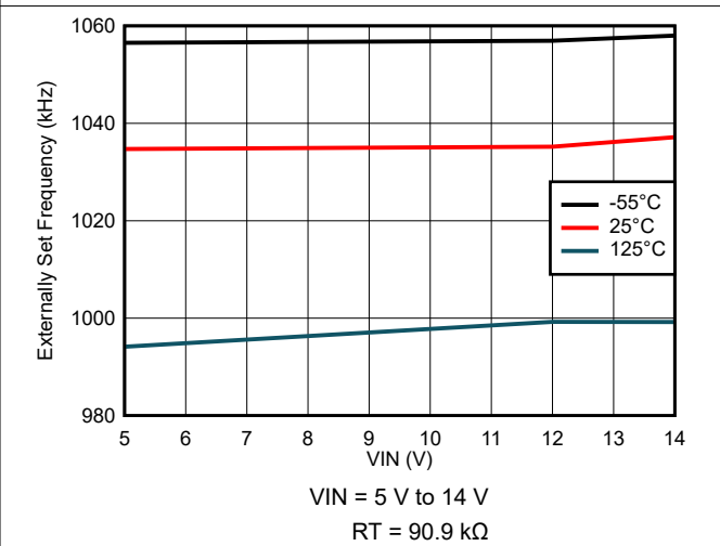
Figure 7-24. Externally Set Frequency Variation
