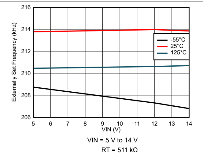
Figure 7-22. Externally Set Frequency Variation
