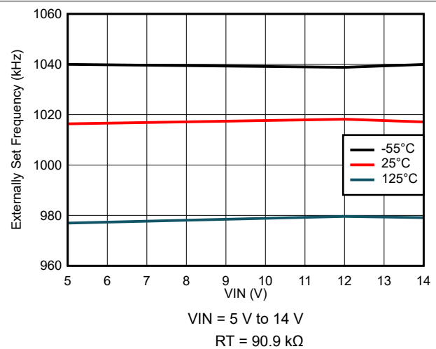
Figure 7-24. Externally Set Frequency Variation
